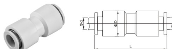
KQ2U 系列-直通 KQ2U Series-Union Straight
